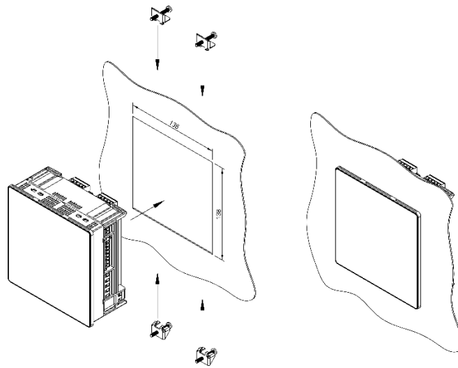
Figure 3.2.1 Installation Diagram
