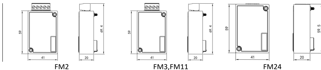
Figure 3.1.2 Extension Module (Unit: mm)
